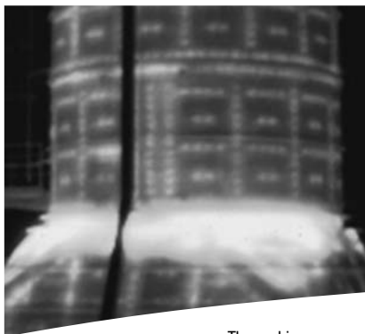
Thermal image of vertical 7F exhaust system.
